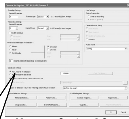
[Camera Settings] Screen
